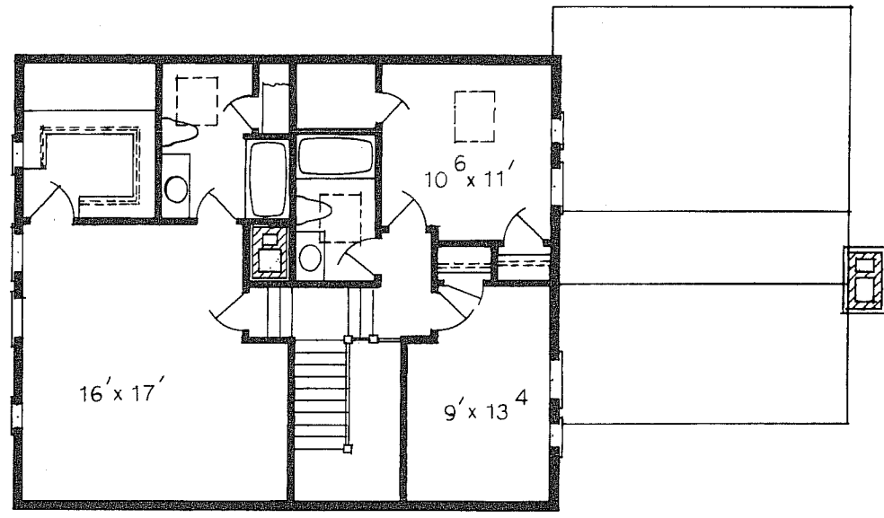
Second Floor
